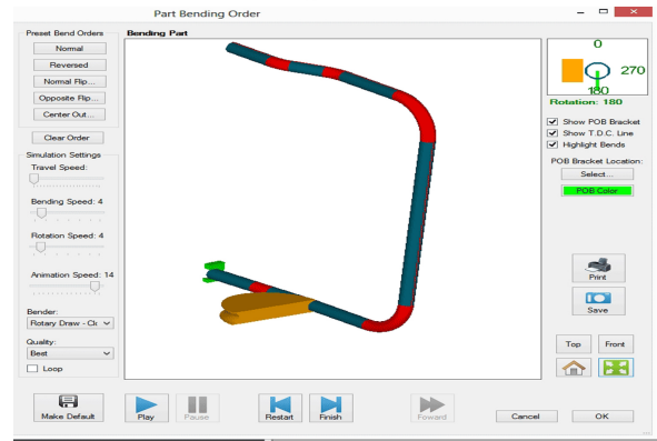
Bending Simulation
